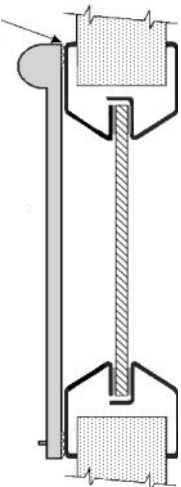
3M Dual Lock® Attachment to Vision Lite
