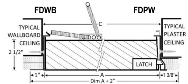
1 HOUR COMBUSTIBLE RATING - CEILING
