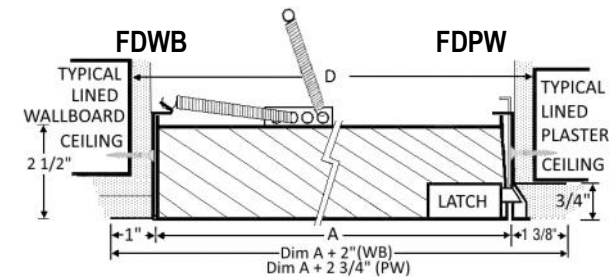
2-3 HOUR NON-COMBUSTIBLE RATING - CEILING
