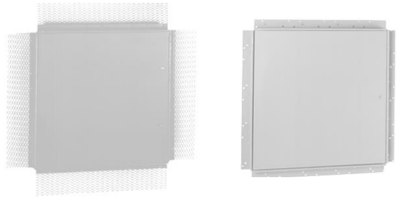
TME - 2 3/4" Plaster Stop with Expanded Metal TMP with 1 3/8" wide Metal Flange
