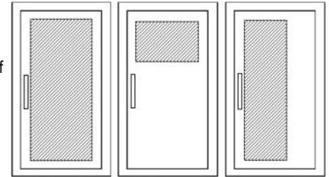
F - Full glass with pull G - Full Glazing with SAF-T-LOK handle and Saf-T-Lok (Not Shown) D - Horizontal duo panel with pull E - Horizontal duo panel with pull and Saf-T-Lok. (Not Shown) V - Vertical duo panel with pull W - Vertical duo panel with pull and Saf-T-Lok. (Not Shown)
