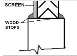
"CORE" Style Mounting
