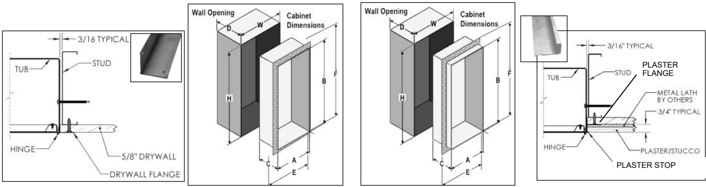
TRIMLESS FLANGE FOR 5/8" DRYWALL
