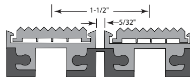
EG602 Cross-Section
