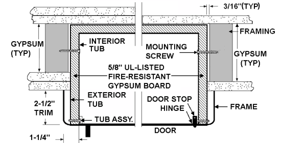
TYPICAL FIRE-RATED INSTALLATION
