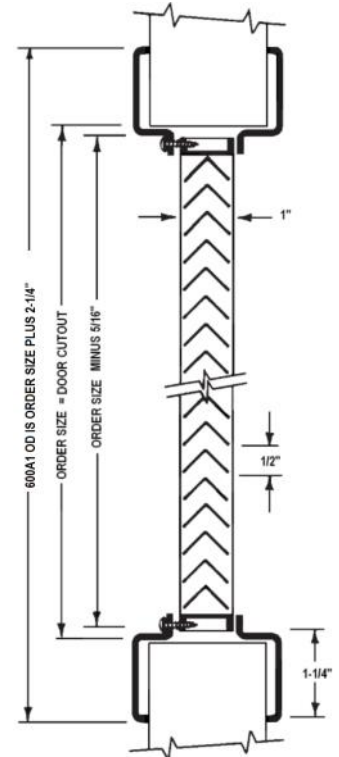
600A1 Self-Attaching Frame Photo & Drawing
