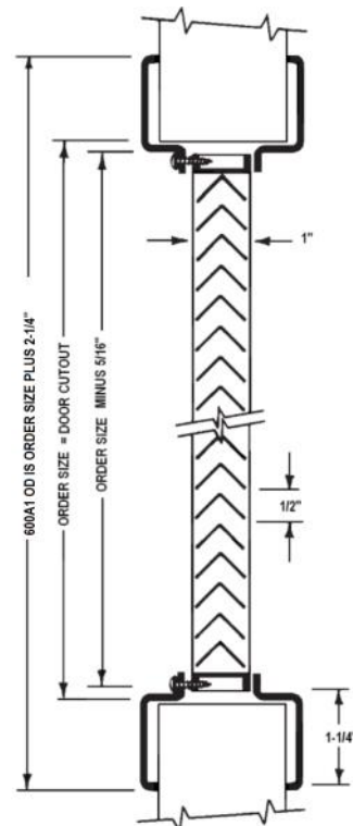
600A1 Self-Attaching Frame Photo & Drawing
