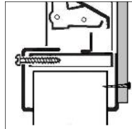
Adjustable Louver Mounting
