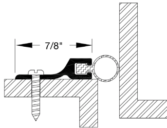
WT-807 Perimeter Weatherstrip Gray Vinyl Insert
