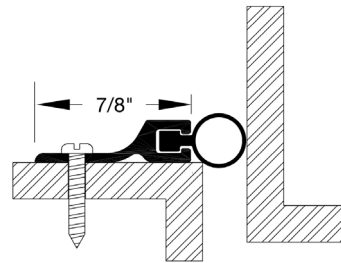
WT-815 Perimeter Weatherstrip Black Polyprene Insert
