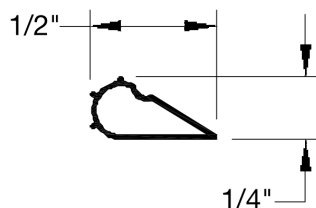
WT-797 Adhesive Gasket Black Polyprene
