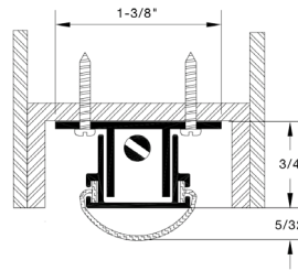
WT-372 Automatic Door Bottom Mortised, Gray Vinyl
